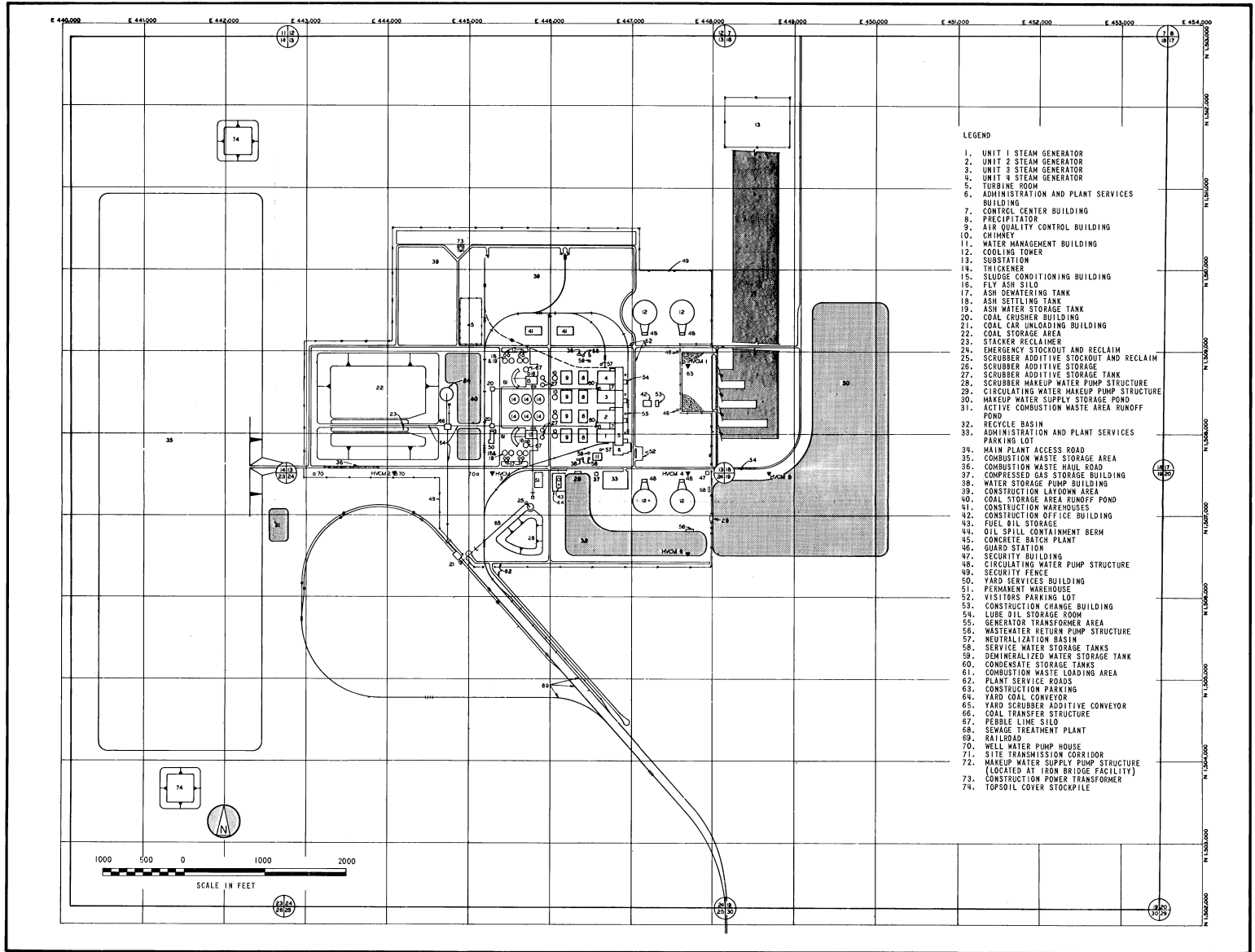
FIGURE 2.1-4. CURTIS H. STANTON ENERGY CENTER FACILITIES ARRANGEMENT-4 UNITS
