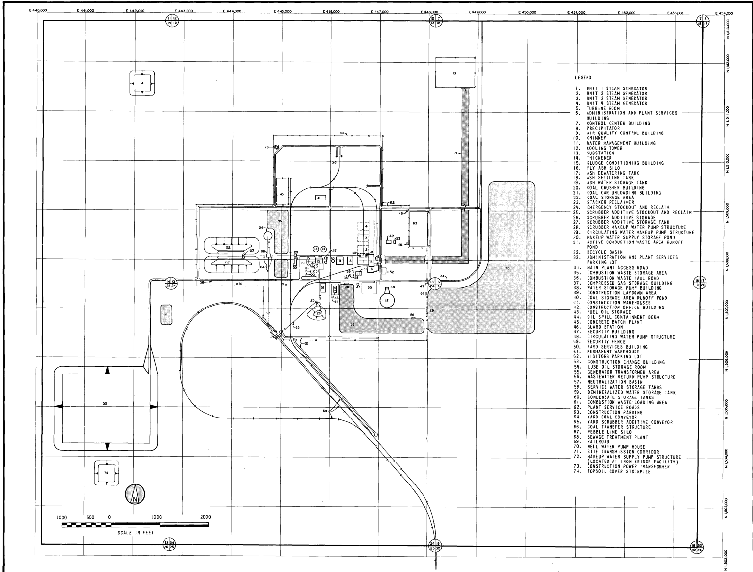
FIGURE 2.1-3. CURTIS H. STANTON ENERGY CENTER FACILITIES ARRANGEMENT-UNIT I
